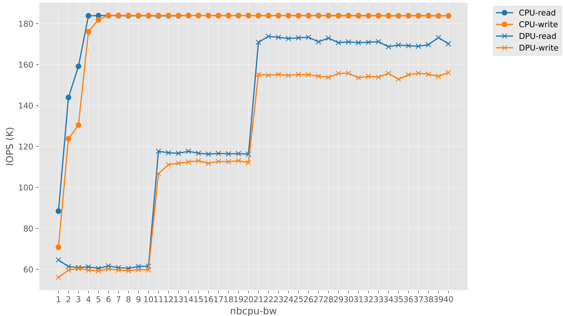
IOPS vs nbcpu-bw (CPU vs DPU)
